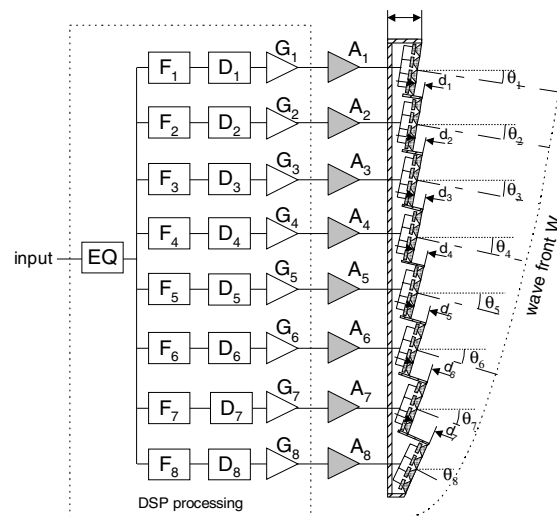
Figure 3 : The DGRC principle
