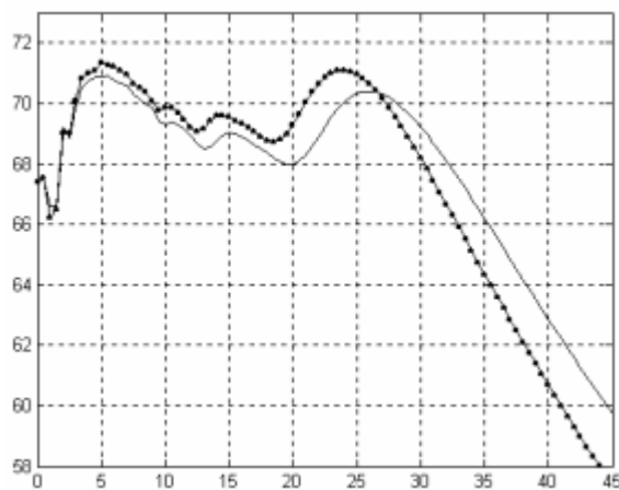
Figure 2 : Perturbation of line array geometry. Line array is 2.4 m high ; its bottom is 1.0 m above the listening plan. Figure plots dB SPL on the listening plan vs distance from the array (m) in the 4kHz octave. Solid curve : loudspeakers at their nominal position. Dotted curve : top of the array tilted forward by 2 cm. Simulation data.
