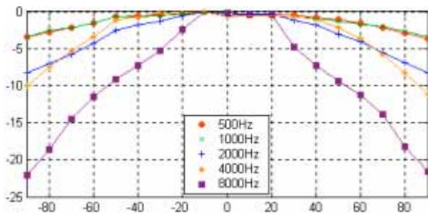
Figure 9 : SPL (dB) per octave vs horizontal angle (deg) measured with column SA250P. Bottom of the column is 2.5 m from the floor. Floor is reflecting. Curves have been normalized to their value at 0°.
