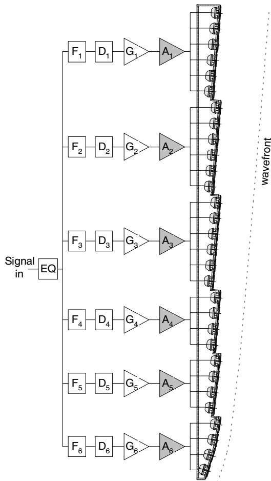
Figure 7 : Same as figure 6, except channels 6 and 7 have been merged into one single channel.
