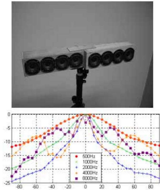
Figure 5 : Directivity of a horizontal DGRC array consisting of 2 sub-arrays of 4 three inches loudspeakers shifted by 36 mm. Signal applied to the right sub-array has been delayed by 104 \mu s. Top : loudspeaker layout. Bottom : Directivity (dB vs deg) per octave band measured at 1.5 m in the horizontal plane.
