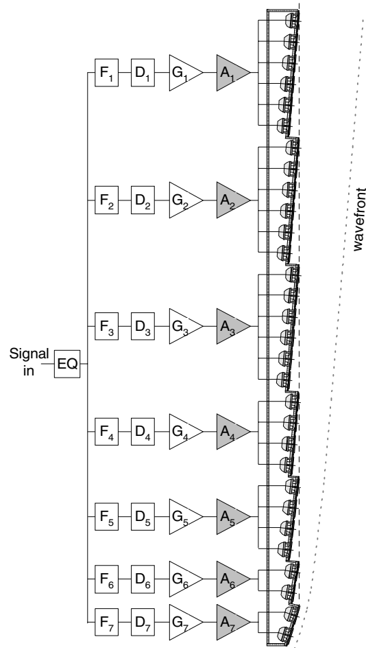
Figure 6 : DGRC array with variable number of loudspeakers per channel. EQ : Equalizer – F_i : Filters – D_i : Delays – G_i : Gains – A_i : power Amplifiers
