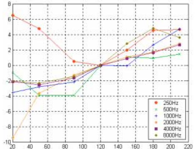
Figure 10 : SPL (dB) per octave vs microphone height (cm) measured with column SA250P. Bottom of the column is 2.5 m from the floor. Floor is reflecting. Curves have been normalized to their value at 120 cm.
