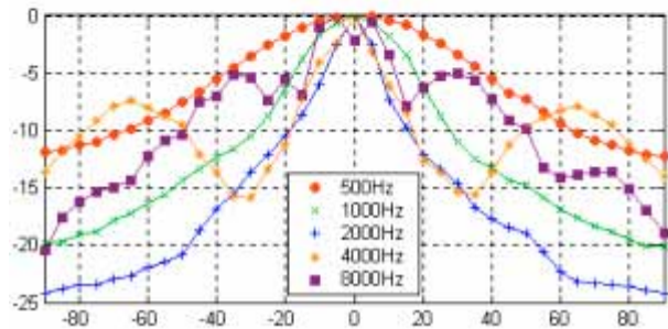
Figure 4 : Directivity of a horizontal linear array of 8 three inches loudspeakers side-by-side.
