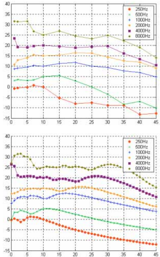
Figure 8 : SPL (dB) per octave vs distance (m) measured with a 2.5m DGRC column. Bottom of the column is 2.5 m from the floor. Microphone is 1.5 m from the floor, in front of the column. Floor is reflecting. Curves have been normalized to their value at 10 m, and shifted for more readability. Top : Measured - Bottom : Predicted.
